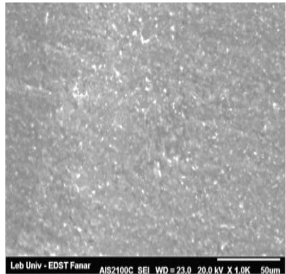
Fig. 7. SEM micrograph of Ceram.x.mono replica before bleaching (1000x magnification).
