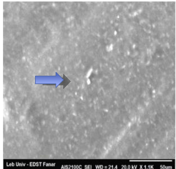
Fig. 6. SEM micrograph of IPS Empress Direct replica one-year after bleaching (1000x magnification).
